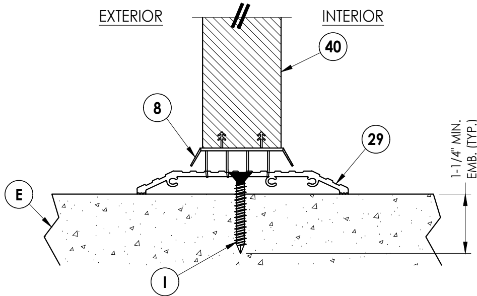
4 VERTICAL CROSS SECTION 6 ADA Inswing configuration
