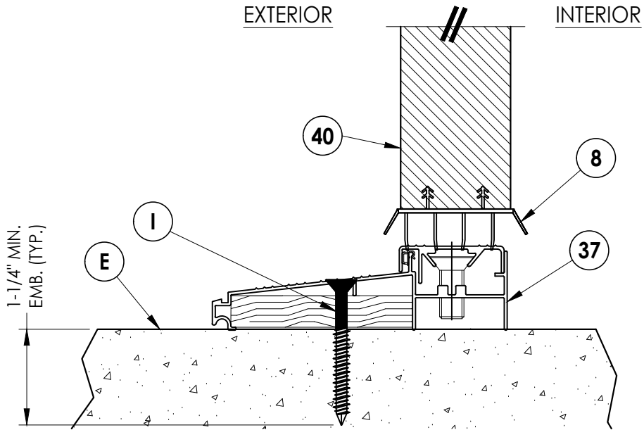
2 VERTICAL CROSS SECTION 6 Inswing configuration
