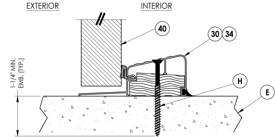
1 VERTICAL CROSS SECTION 6 Outswing configuration
