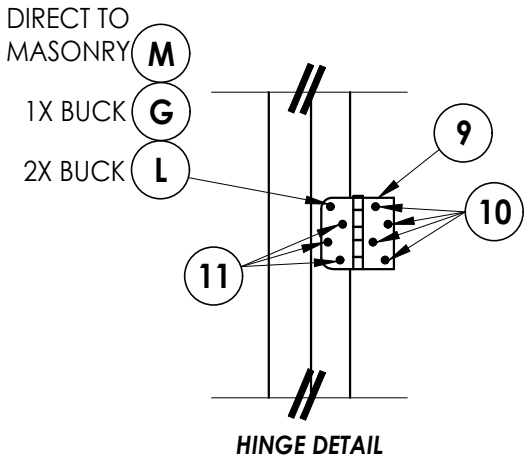
HINGE DETAIL
