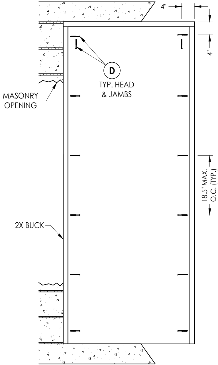
BUCK ANCHORING
