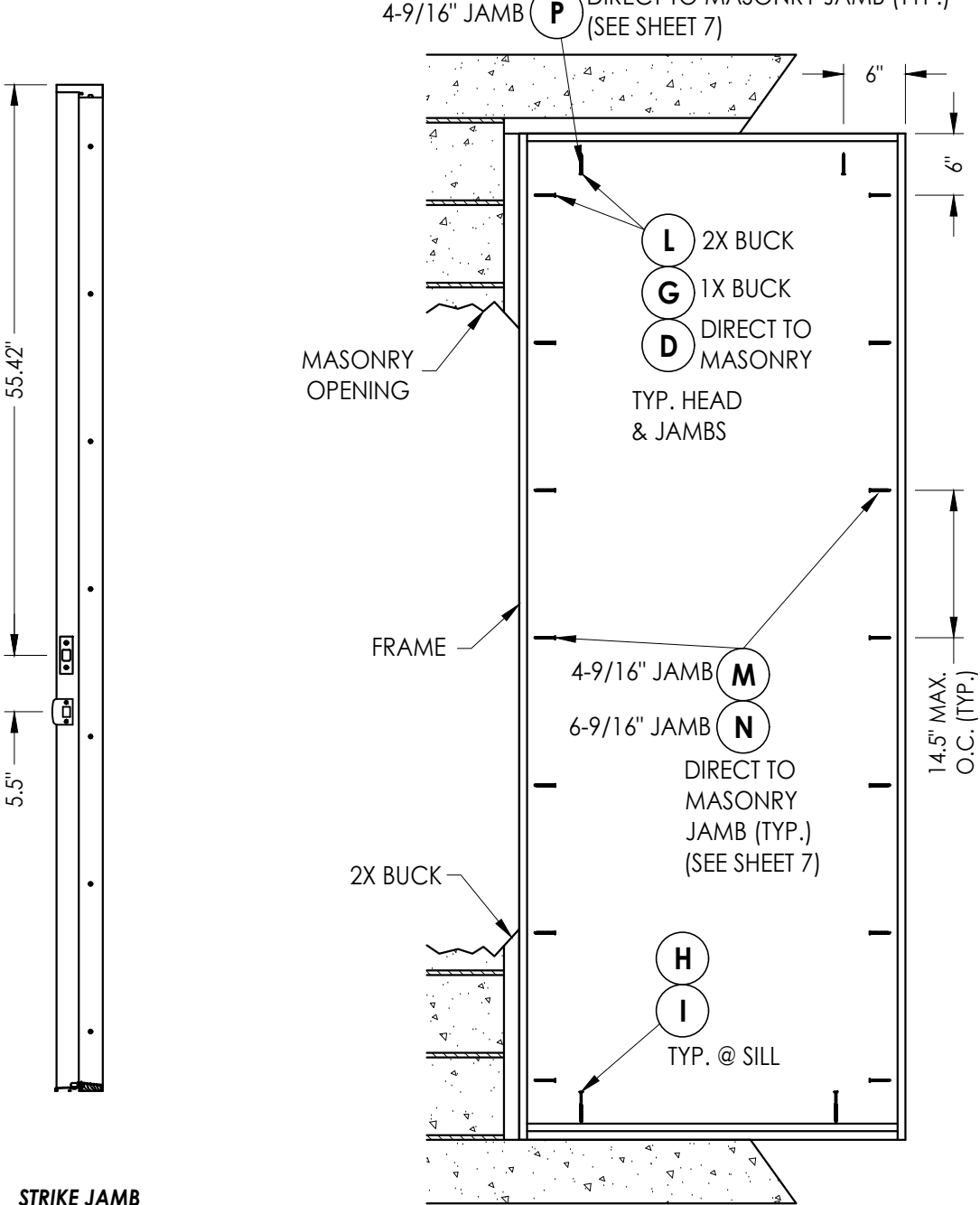
FRAME ANCHORING
